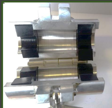
Fig 2. Viper MRC with guide bushes.
